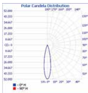
Vaya Flood HP 3000K, 20deg
