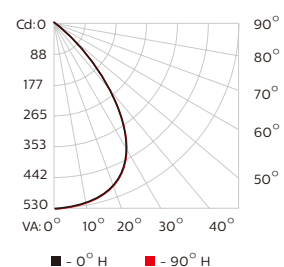
RGB, 80° diffuser lens
