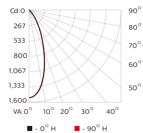
RGB, 40° diffuser lens
