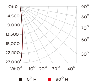
RGB, 8° native lens
