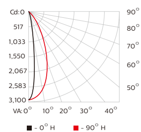
RGB, 10° x 40° asymmetric lens
