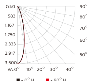
RGB, 20° diffuser lens
