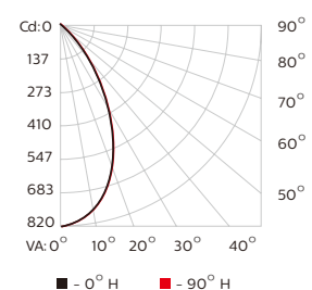
RGB, 60° diffuser lens
