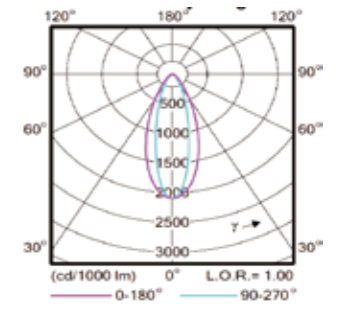
A4: 25x40° Beam Angle
