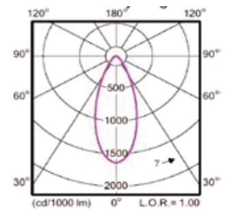
50x50° Beam Angle
