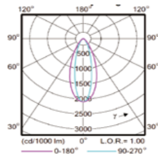
A4: 25x40° Beam Angle
