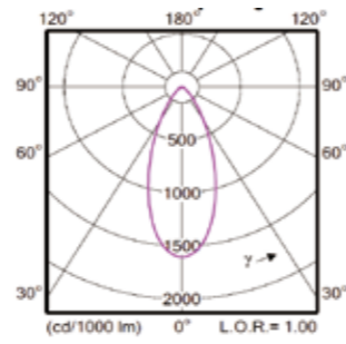
40x40° Beam Angle
