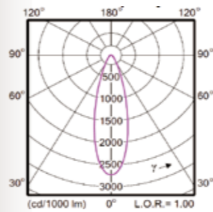
30x30° Beam Angle
