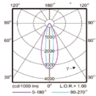
A2: 16x35° Beam Angle
