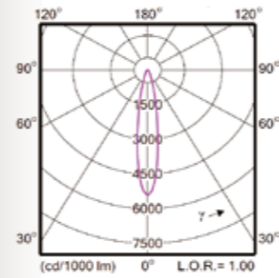
17x17° Beam Angle
