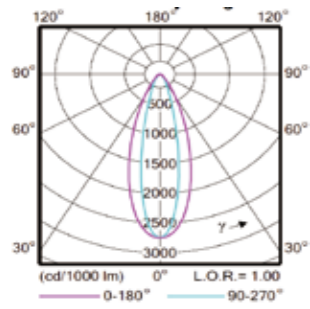
A3: 20x40° Beam Angle
